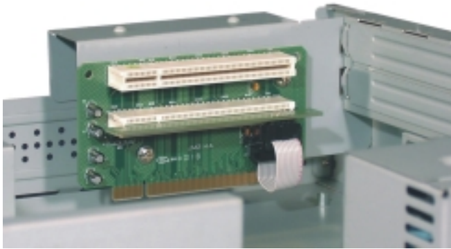
Riser Card in PCI Version
